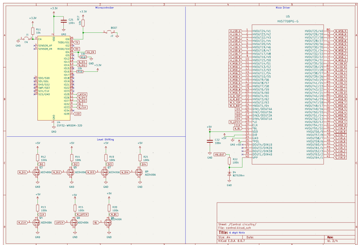
Figure 5: Sub-circuit sheet
