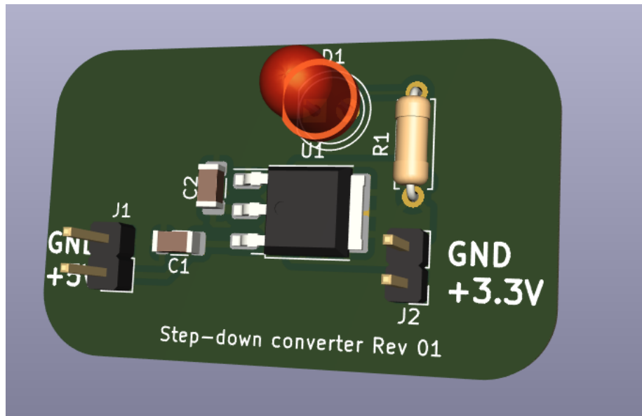
Figure 12: 3D-view
