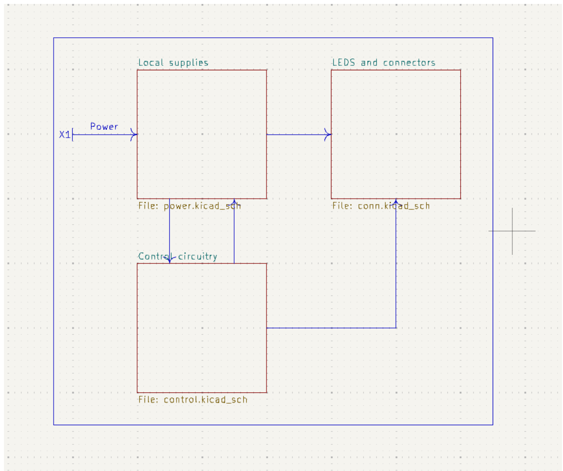
Figure 4: Root sheet
