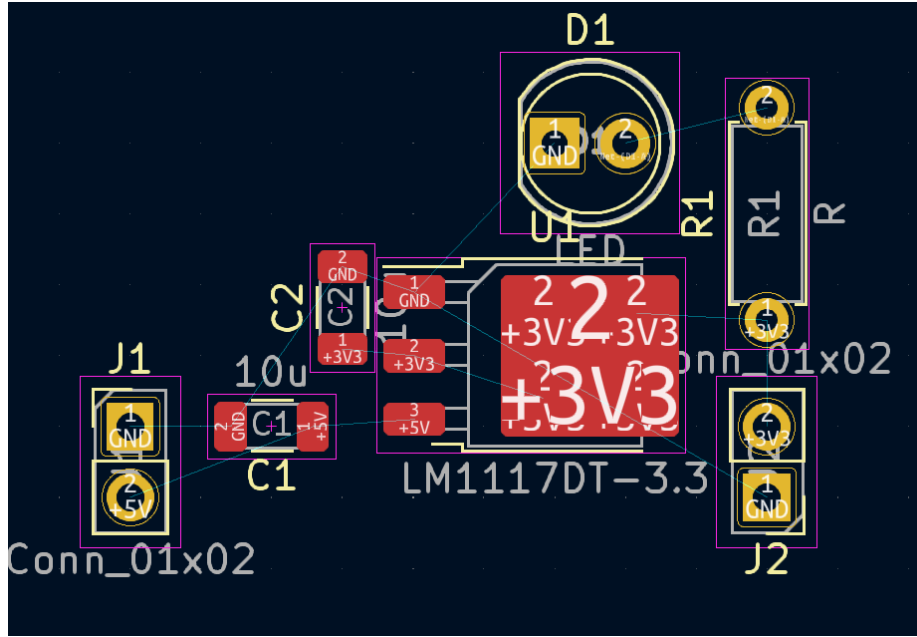
Figure 9: Placement of components
