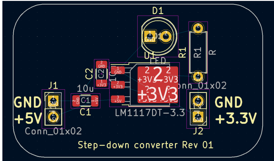
Figure 10: Text and edge placement
