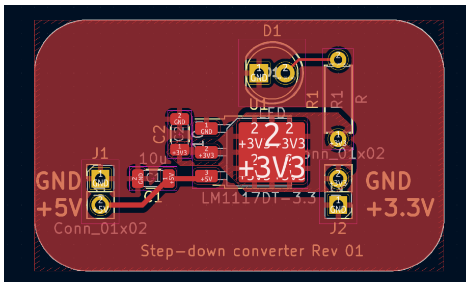
Figure 11: Final PCB
